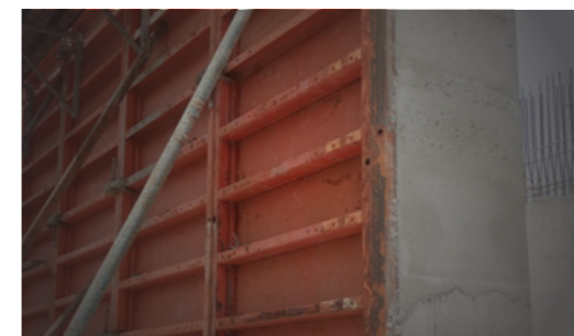
Steel Formwork Forming Effect
